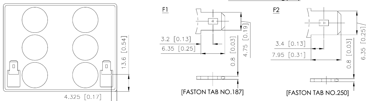
Detail A Drawing(3:1)
